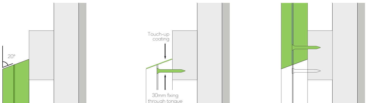
Fig. 18 - Joining boards detail
